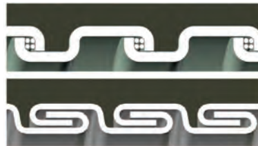
Square-Locked Design with cord packing 3/8" - 1-1/4"
